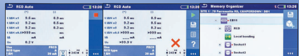
RCD Auto Test PASS Result
