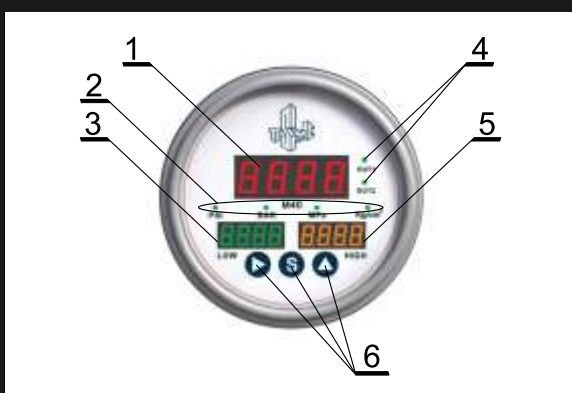
Figure 1-1 Pressure/vacuum meter's panel
