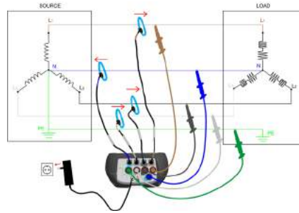
Connection to 3-phase 4-wire system
