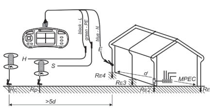
Circuits for three-wire measurement
