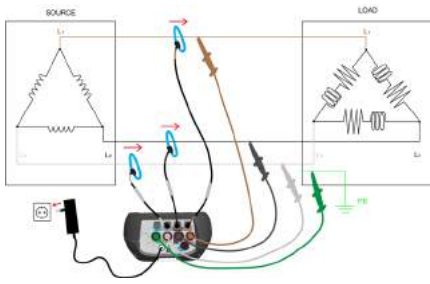
Connection to 3-phase 3-wire system
