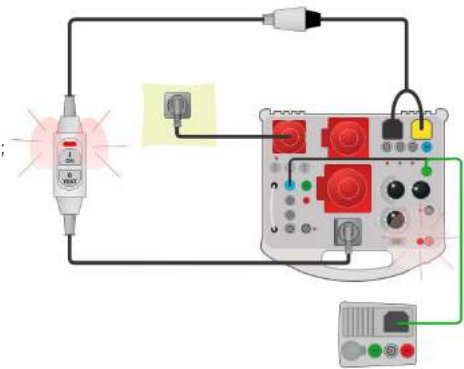
Testing the continuity of the protective earth conductor.
