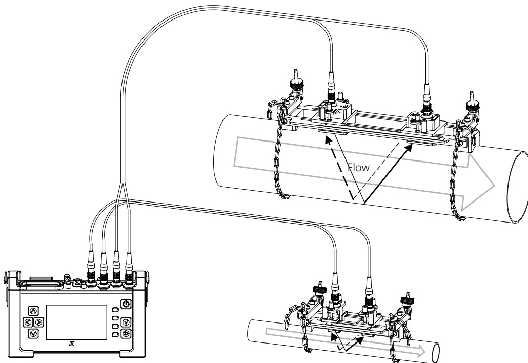
Flow / mass measurement configuration (two pipes at the same time )
