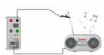
Touch leakage current test for Class II device
