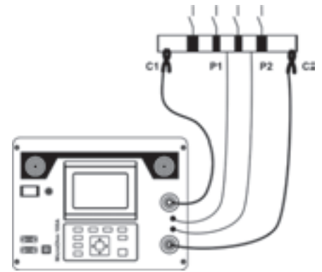
Bus bar connection
