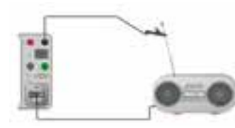
Substitute leakage test for Class II device
