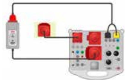
Testing the 3-phase PRCD
